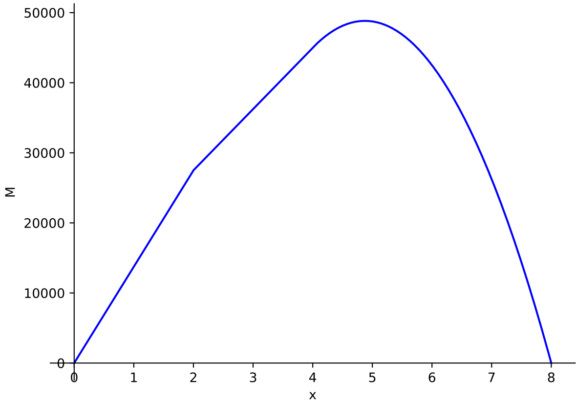
Bending Moment
